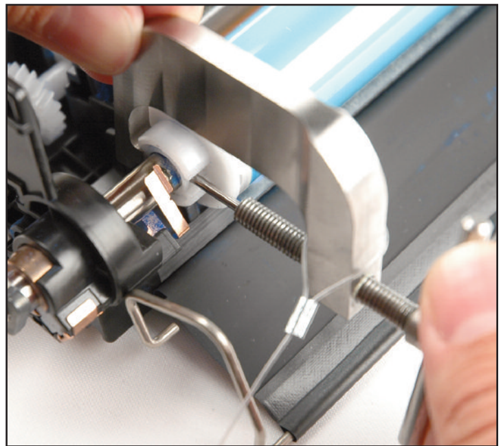
Tool Aligning Color Cartridge Spring Pin
